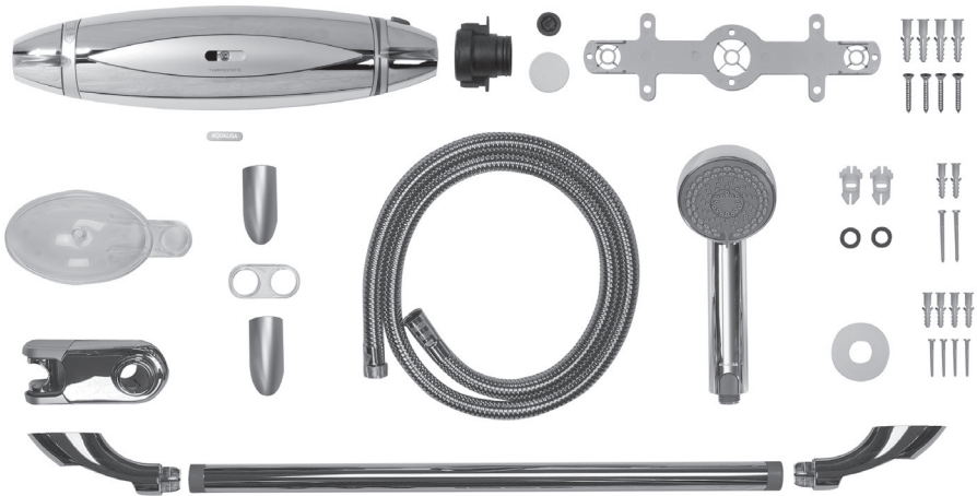
Exposed shower valve with adjustable height Harmony head
